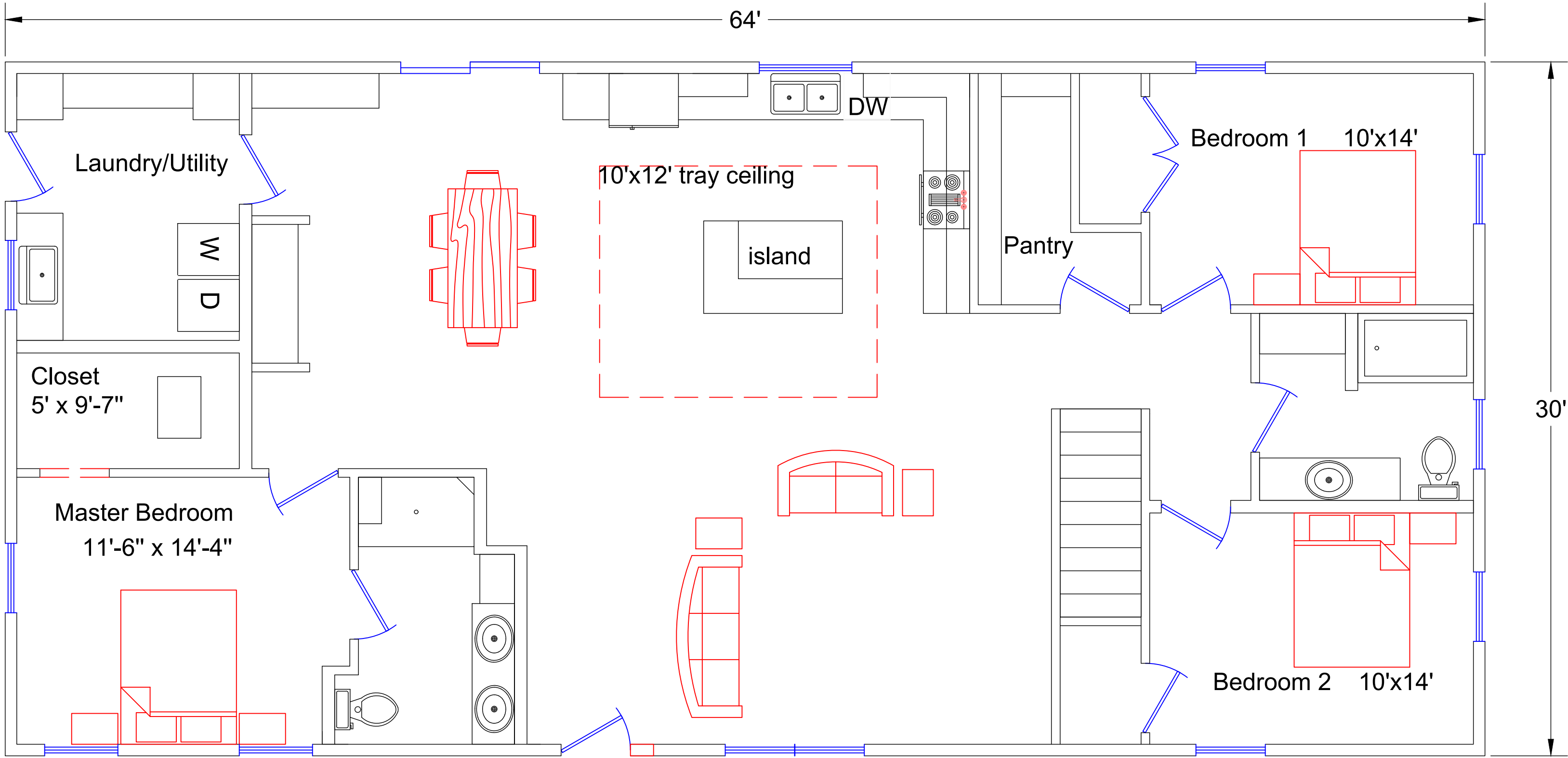
2024-25 Tech house \frac{1}{4}"=1'
